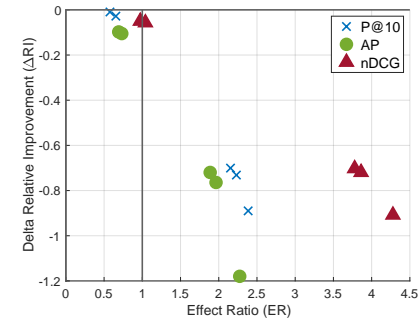
(b) rpd_C runs.
