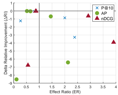
(a) rpd_tol runs.
