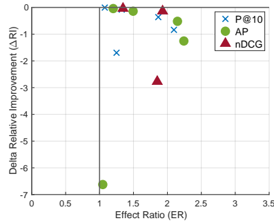
(a) rpl_tol runs.
