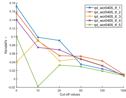
(a) Kendall's \tau WCrusbust0405.
