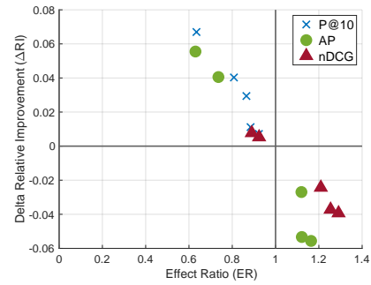
(b) rpl_C runs.
